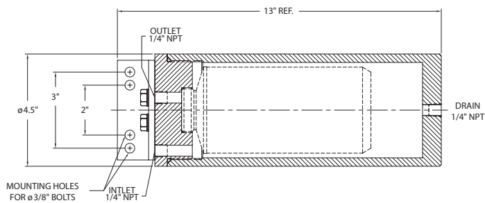
F-4 FILTER/DRYER
