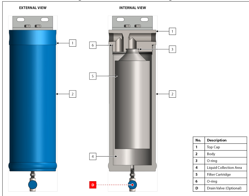
Figure 2: F-31 Maintenance Diagram
